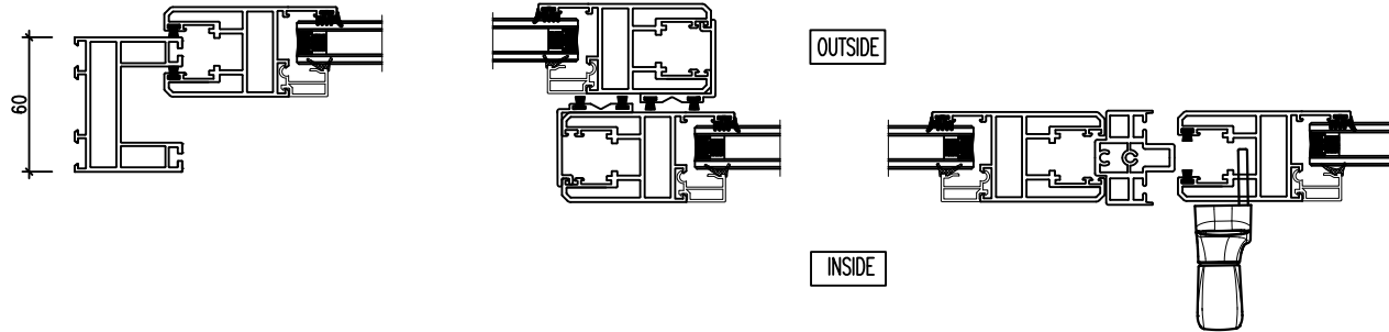
B SECTION DETAIL
